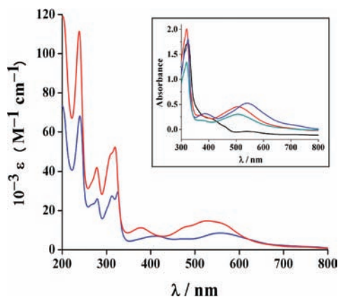
Figure 4. Electronic spectra of 1 (blue) and 2 (red) in \text{CH}_3\text{CN} . Inset: Electronic spectra of [\text{Ru}(\text{trpy})(\text{L})(\text{Cl})]^+ ( 1 , blue), [\text{Ru}(\text{trpy})(\text{L})(\text{EtOH})]^+ (green), 1 in the presence of \text{H}_2\text{O}_2 , i.e., in situ generated [\text{Ru}(\text{trpy})(\text{L})(\text{O})]^+ ( 3 , black), and 3 + \text{PPh}_3 (Red) in EtOH.
